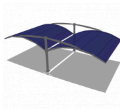
X-11 Solar Eclipse
